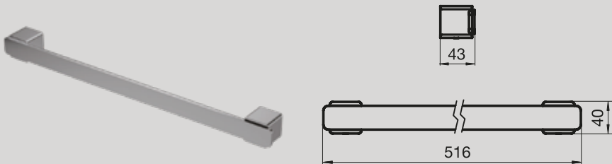
FV164/J5 Barral 450 mm. PC-FB
