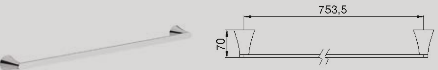
FV164.02/K4 Barral 760 mm. PC-BB-BG-BK-BN PB-BHB-UPB-PN-SGR
