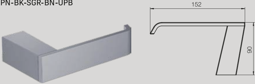
FV167/J8 Portarrollo. BB-BG-PB-PC-BHB PN-BK-SGR-BN-UPB
