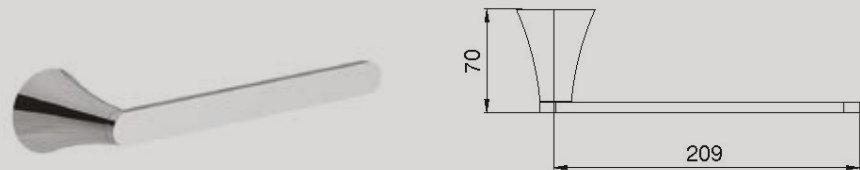
FV163/K4 Toallero corto. PC-BB-BG-BK-BN PB-BHB-UPB-PN-SGR
