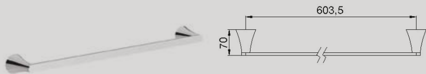
FV164.01/K4 Barral 600 mm. PC-BB-BG-BK-BN PB-BHB-UPB-PN-SGR
