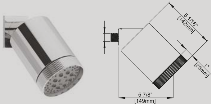
FV126/J2V Flor de ducha. PC-BB-BG- BK-BN-PB UPB-BHB- PN-SGR
