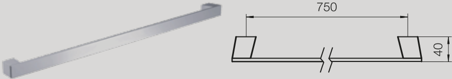
FV164.02/J8 Barral 750 mm. BB-BG-PB-PC-BHB PN-BK-SGR-BN-UPB
