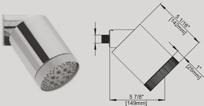
FV126/J2K Flor de ducha. PC-BB-BG- BK-BN-PB UPB-BHB- PN-SGR
